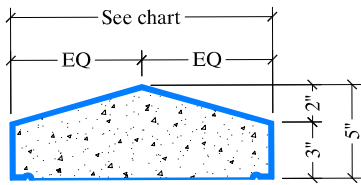
PIER CAP (PC1)
